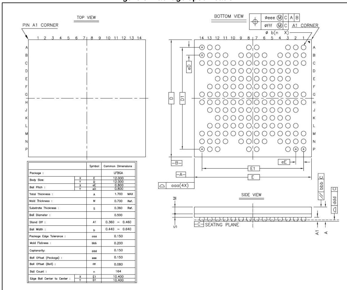
Figure 3. Package specification
