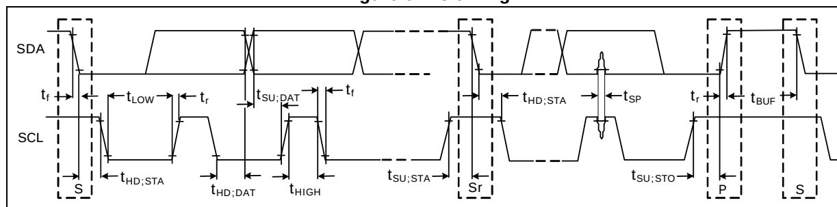
Figure 6. I 2 C timing
