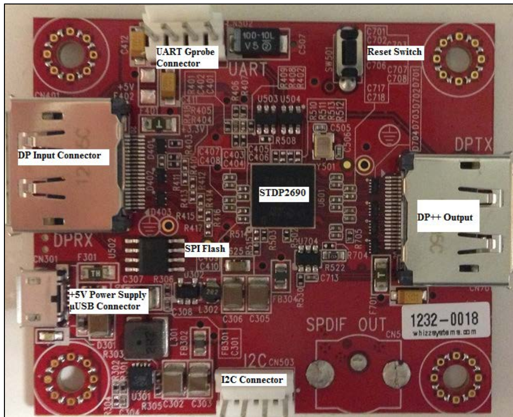
Figure 3. Board picture
