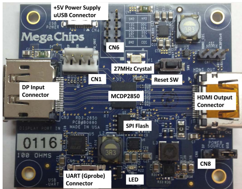
Figure 1. Board picture
