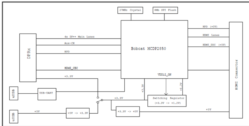
Figure 3. Connection diagram
