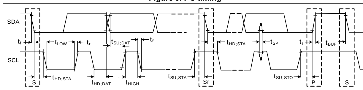
Figure 9. I2C timing
