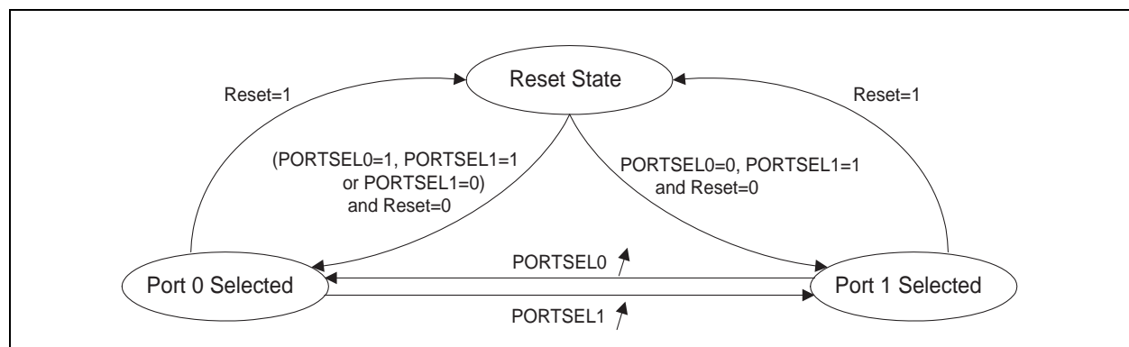
Figure 2. Reset State Machine (Edge-Sensitive Sideband Mode)
