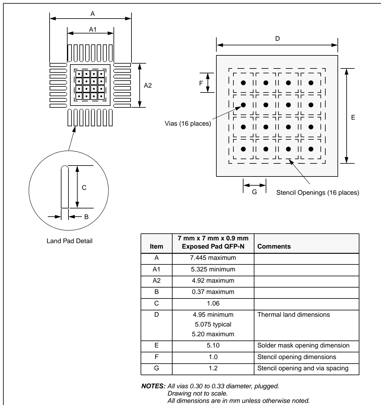
Figure 11. Recommended Land Pattern
