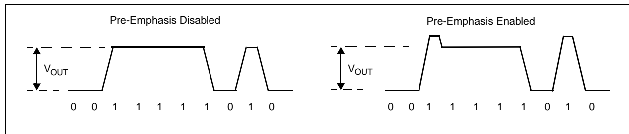
Figure 5. Pre-Emphasis Diagram
