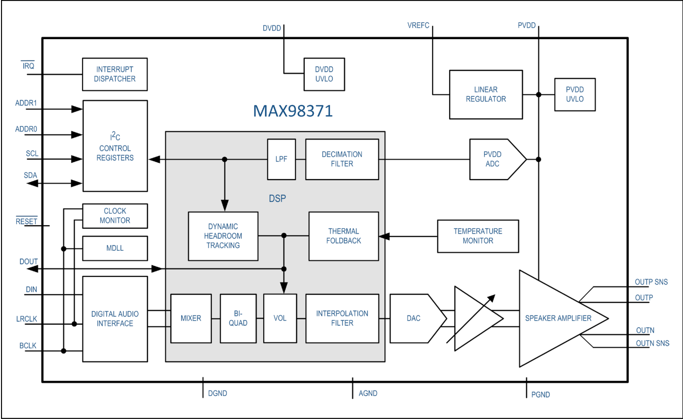
Detailed Functional Diagram
