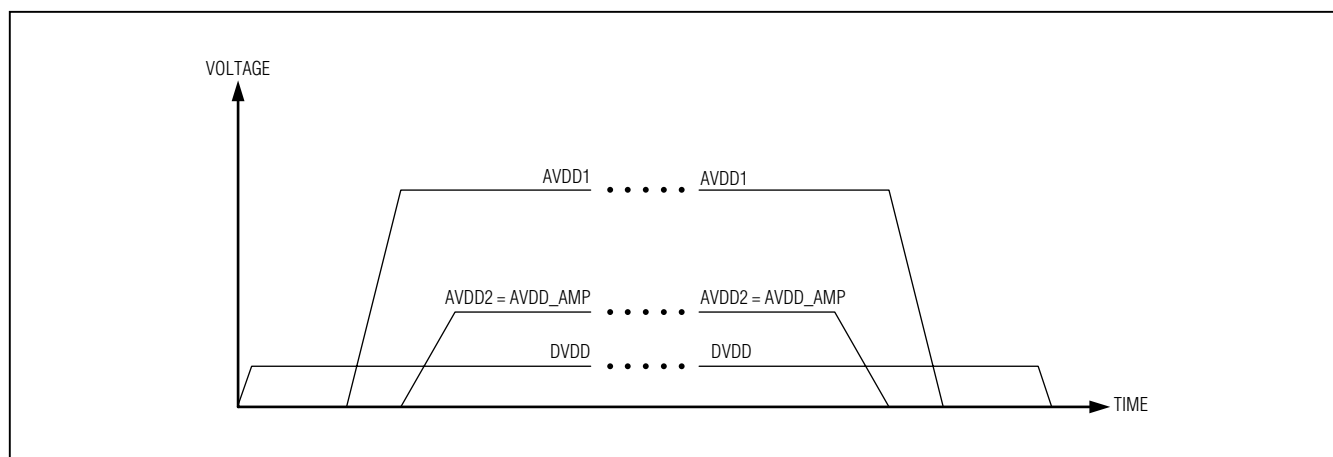
Figure 15. Power-Up and Power-Down Sequence with AVDD2 and AVDD_AMP Connected to Half AVDD
