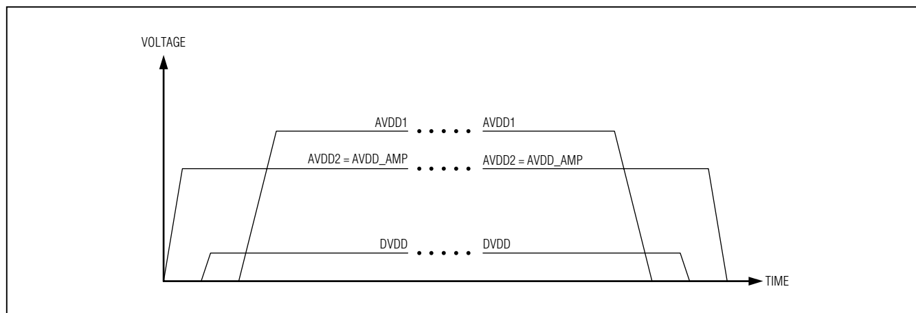
Figure 16. Power-Up and Power-Down Sequence with AVDD2 and AVDD_AMP Connected to 12V
