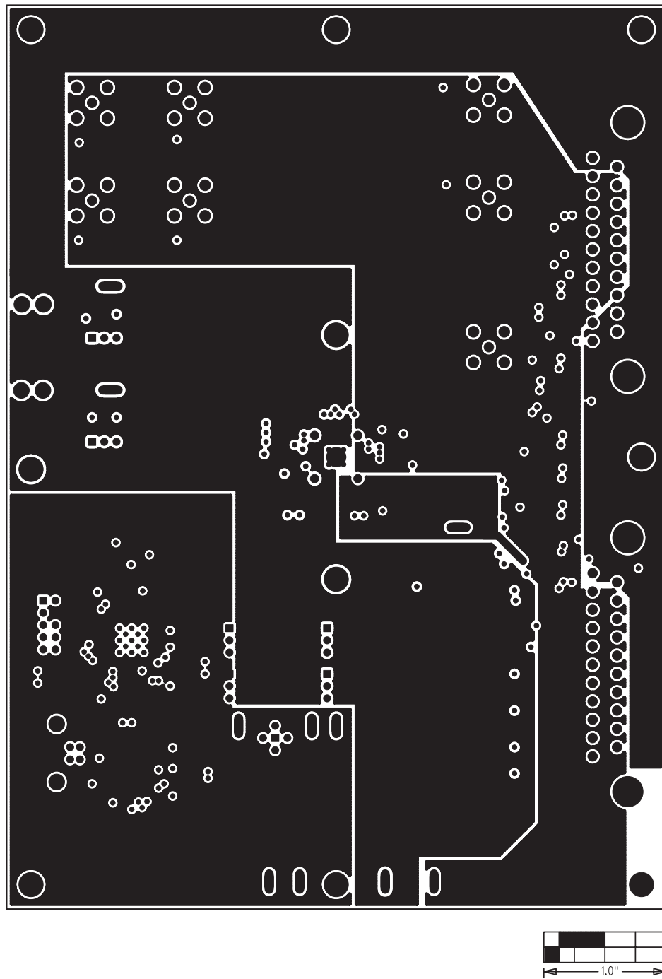
Figure 9. MAX9670 EV Kit PCB Layout—Inner Layer 3
