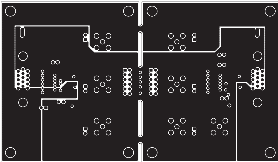
Figure 5. MAX9539/40 EV Kit PCB Layout—PWR Layer 3
