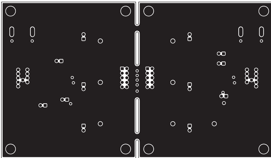
Figure 4. MAX9539/40 EV Kit PCB Layout—GND Layer 2
