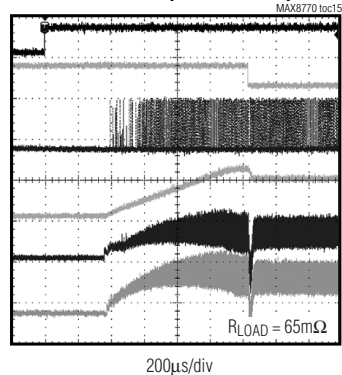
SOFT-START (UP TO \overline{CLKEN} )
