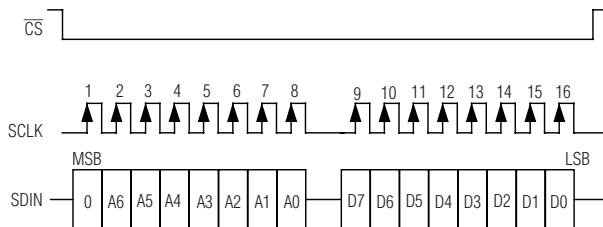
Figure 15. Write Operation
