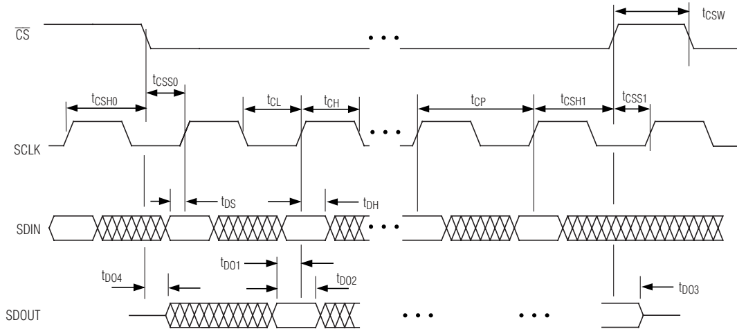
Figure 14. Detailed Serial-Interface Timing
