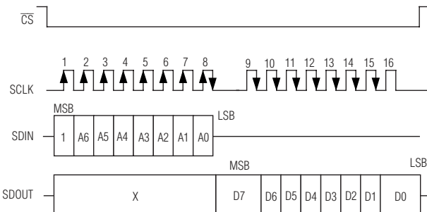
Figure 16. Read Operation
