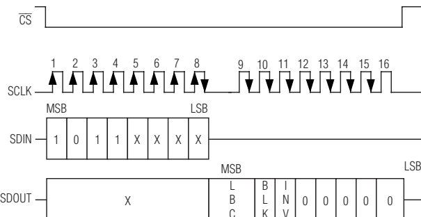
Figure 18. Reading Character Attribute Byte in 8-Bit Operation Mode
