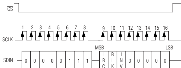
Figure 17. Writing Character Attribute Byte in 8-Bit Operation Mode
