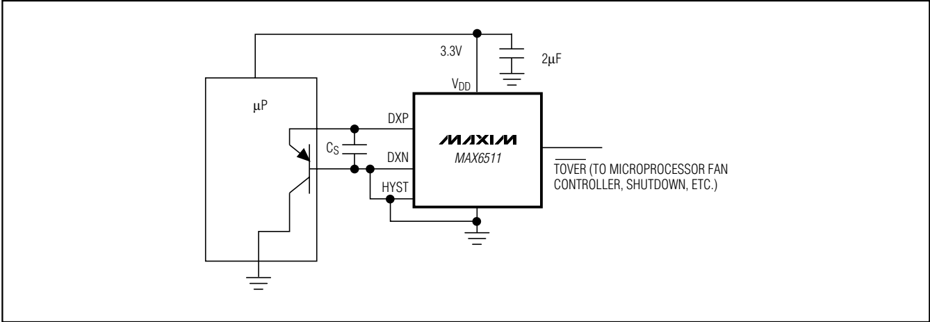
Typical Operating Circuit
