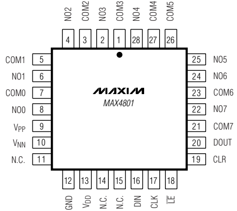
PLCC
