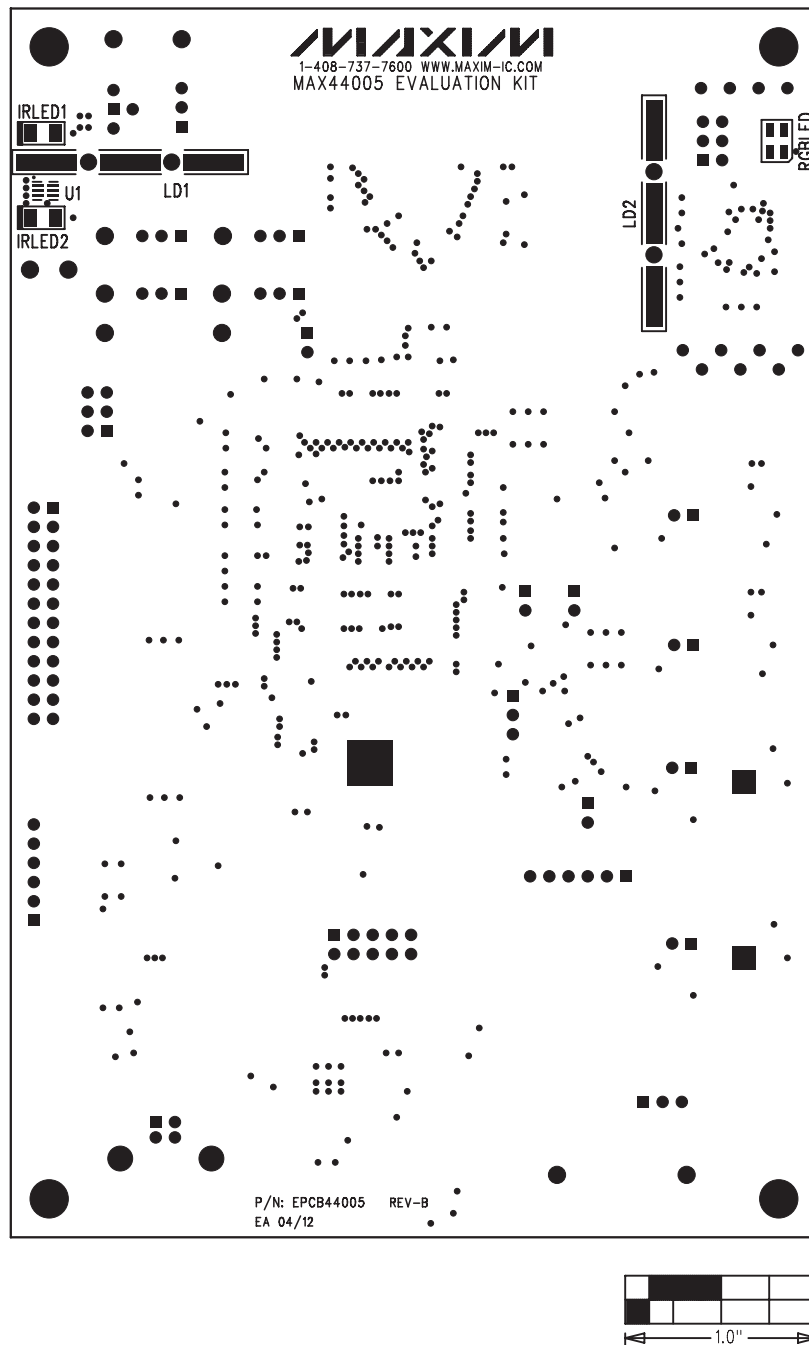
Figure 7. MAX44005 EV Kit Component Placement Guide—Component Side
