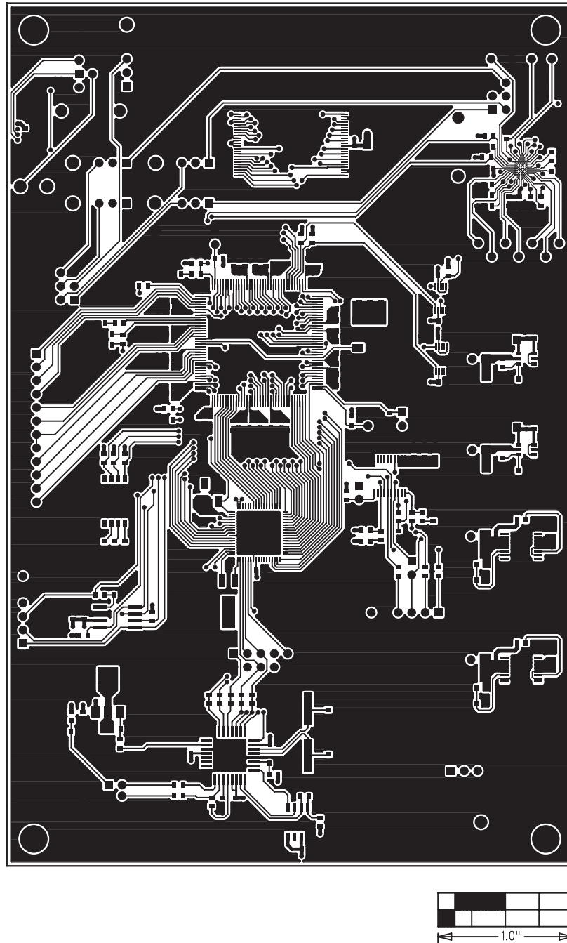
Figure 11. MAX44005 EV Kit PCB Layout—Bottom Side
