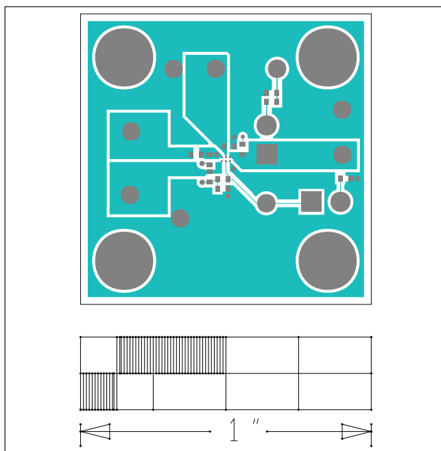
MAX40001 EV Kit—Top
