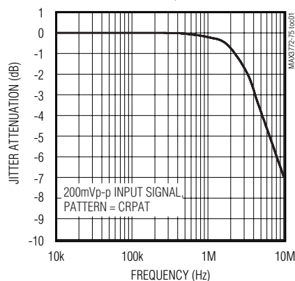
2.125Gbps JITTER TRANSFER vs. FREQUENCY
