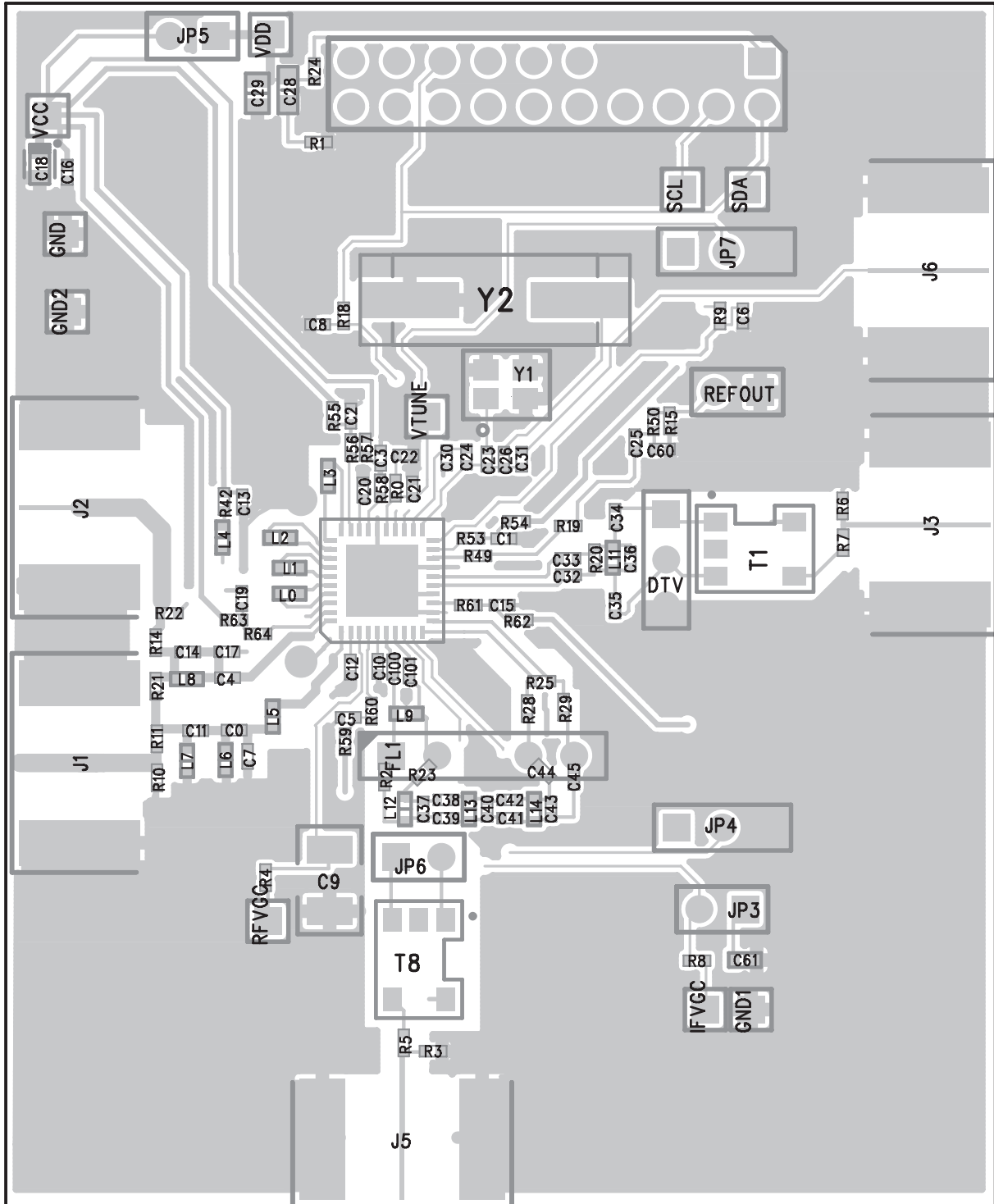
Figure 2. MAX3544 EV Kit Component Placement Guide—Component Side
