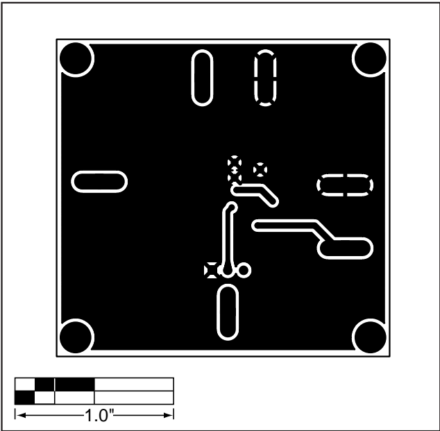
Figure 4. PC Board Layout—Solder Side
