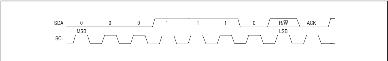
Figure 10. Slave Address
