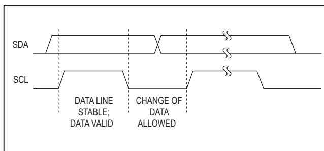
Figure 8. Bit Transfer
