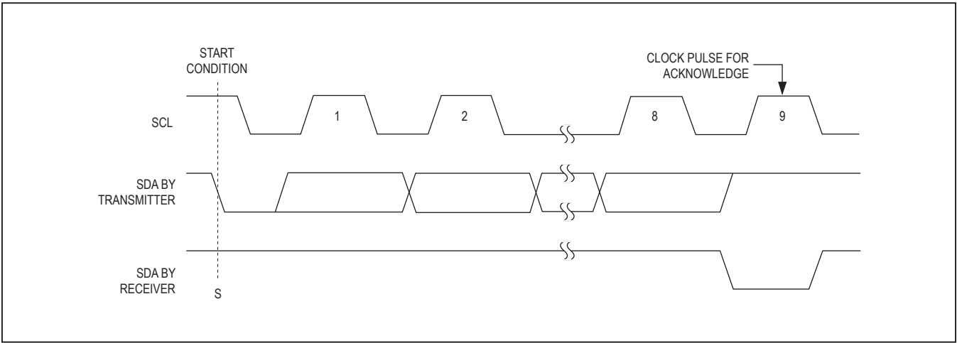
Figure 9. Acknowledge
