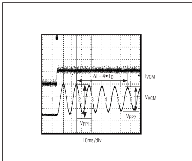
Figure 5. Step Response of Sample VCM
