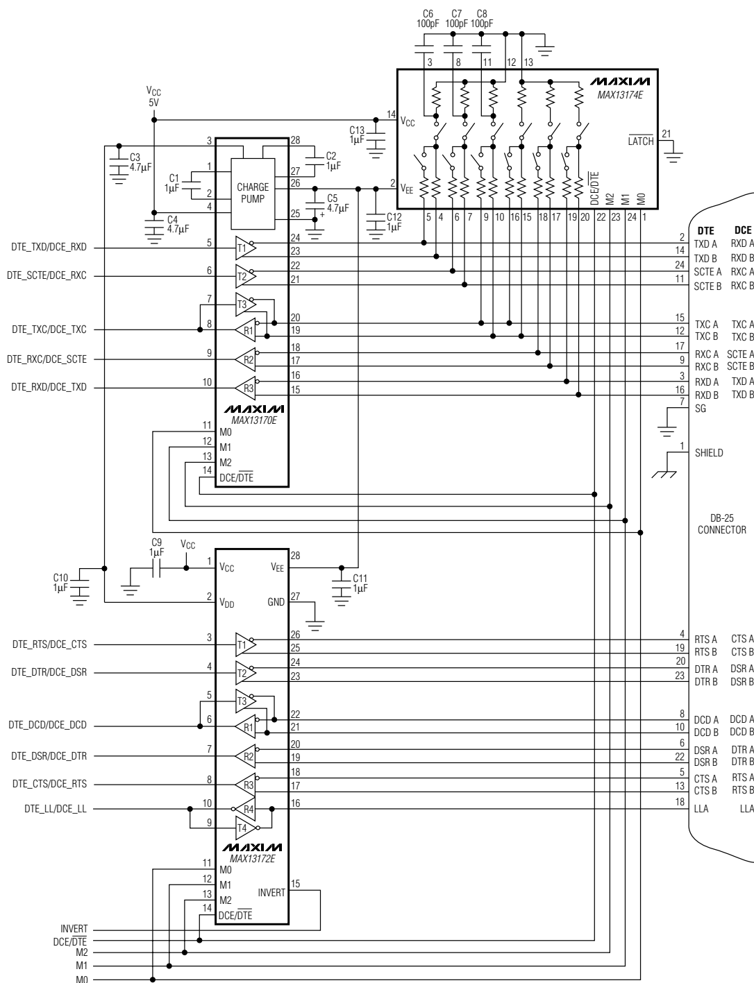
Figure 19. Controller-Selectable Multiprotocol DCE/DTE Port with DB-25 Connector
