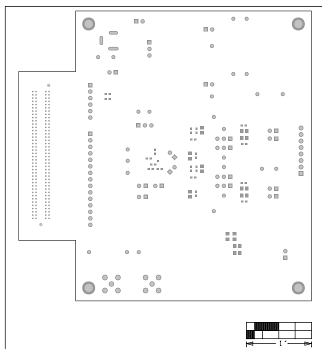
MAX1192 EV Kit—Bottom Mask
