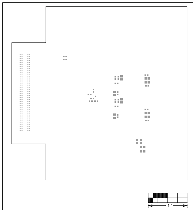
MAX1192 EV Kit—Bottom Paste
