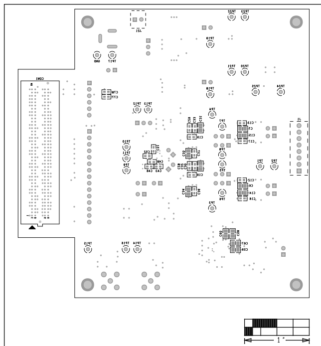
MAX1192 EV Kit—Bottom Silkscreen
