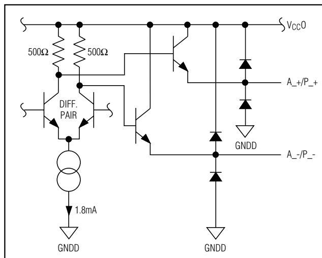
Figure 5. Simplified PECL Output Structure
