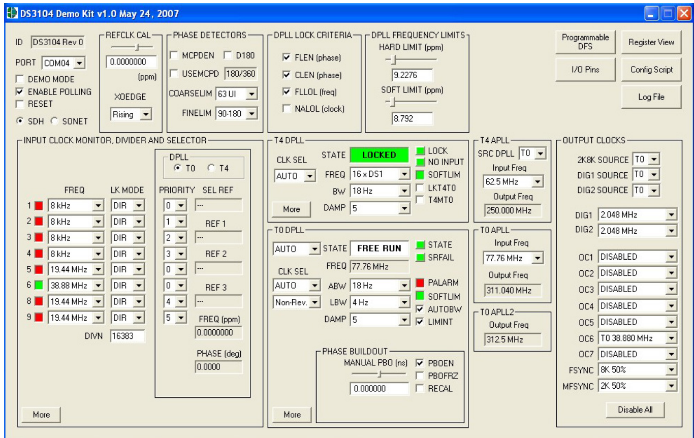
Figure 4-1. Software Main Screen
