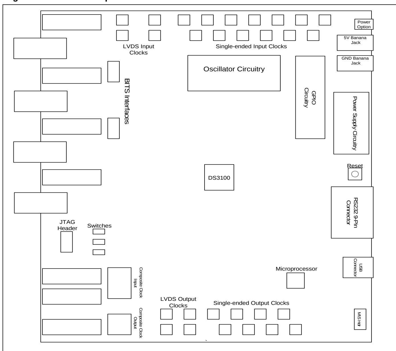
Figure 1-1. Board Floorplan
