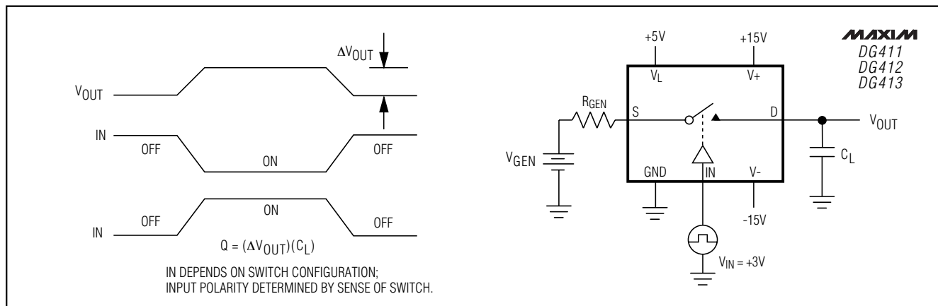
Figure 4. Charge-Injection
