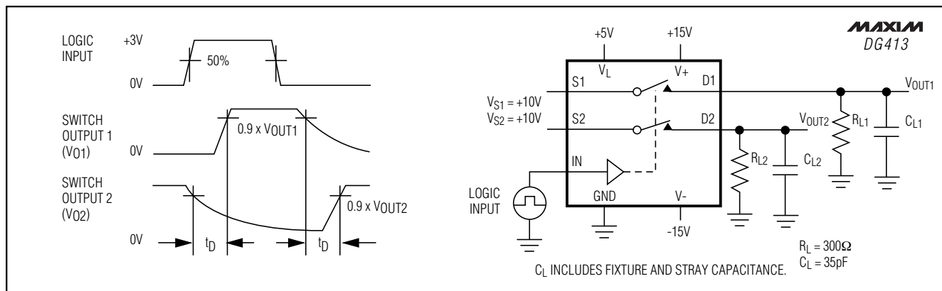
Figure 3. DG413 Break-Before-Make
