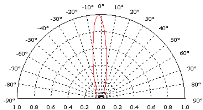
RADIATION PATTERN
