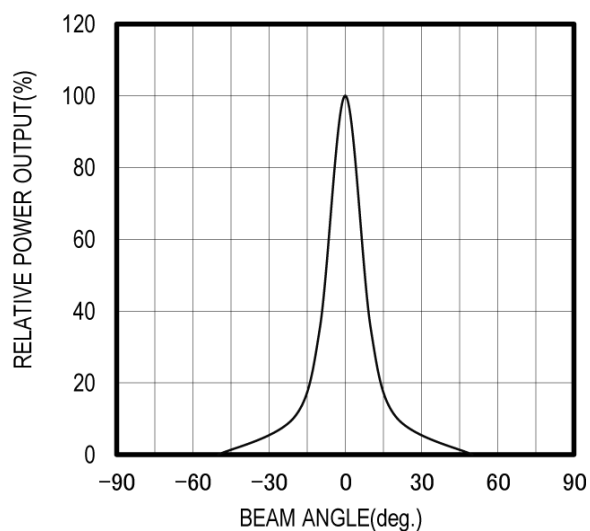
RADIATION PATTERN
