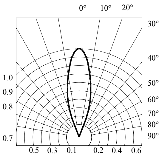
RADIATION DIAGRAM
