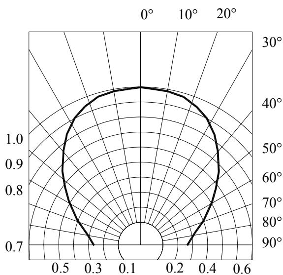
RADIATION DIAGRAM
