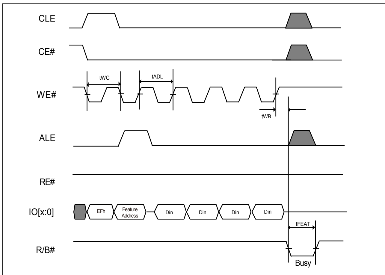
Figure 26. AC Waveforms for Set Feature (ONFI) Operation
