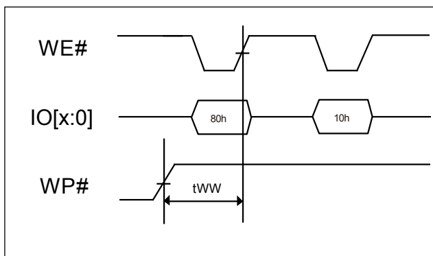
Figure 39-1. Enable Programming of WP# Signal
