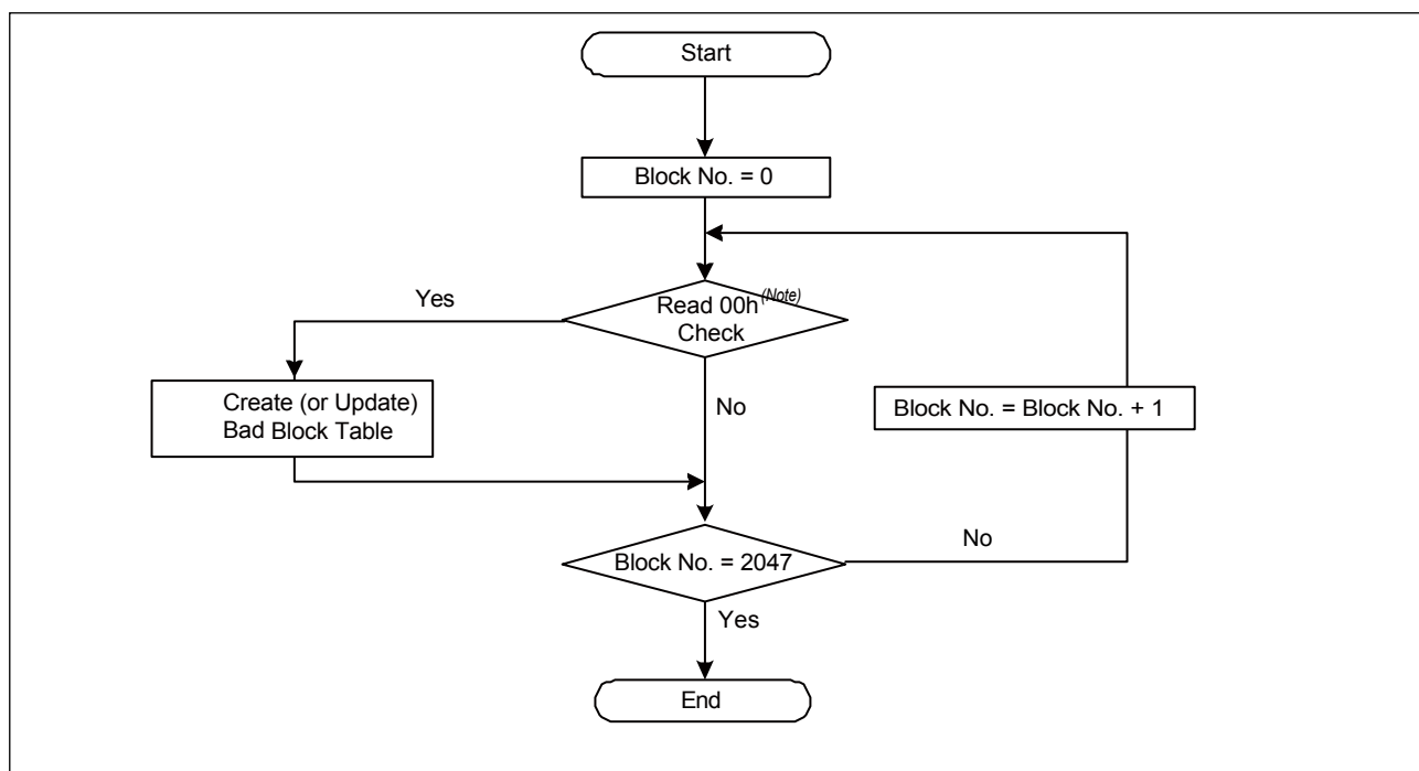
Figure 41. Bad Block Test Flow
