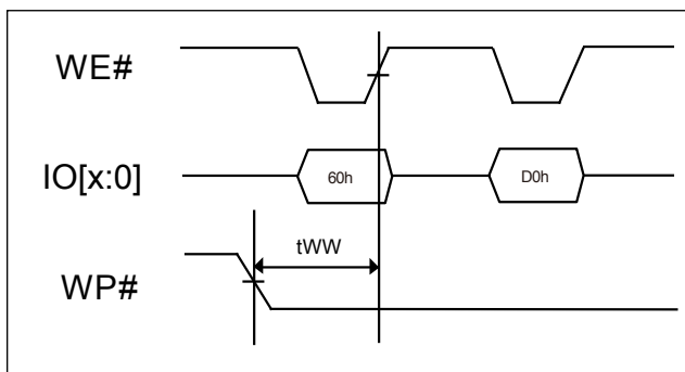
Figure 39-4. Disable Erasing of WP# Signal
