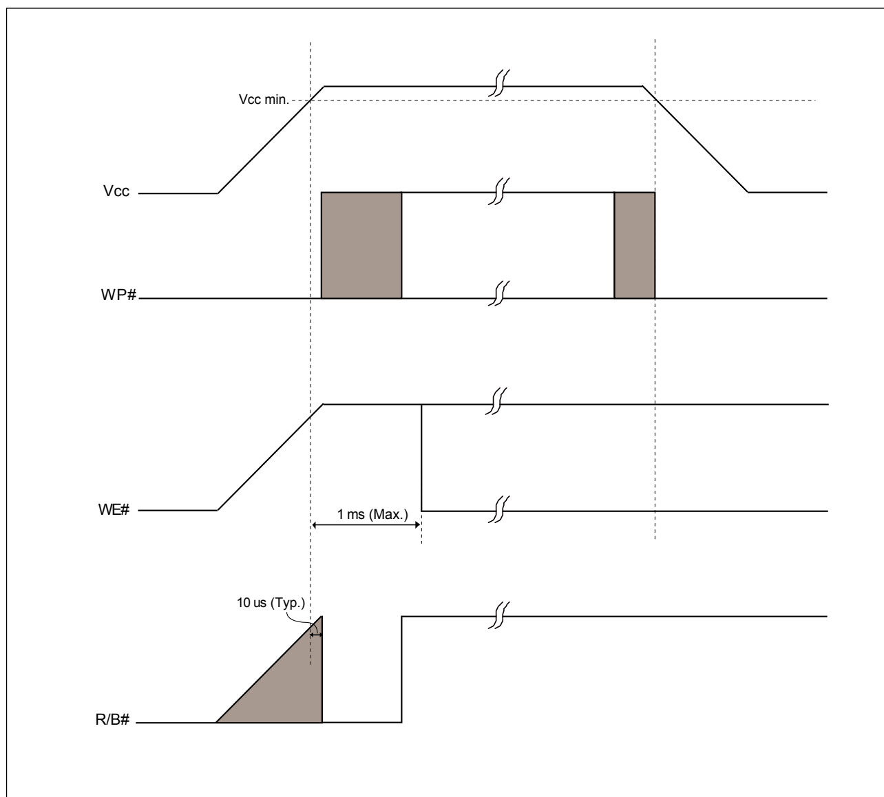
Figure 38. Power On/Off Sequence
