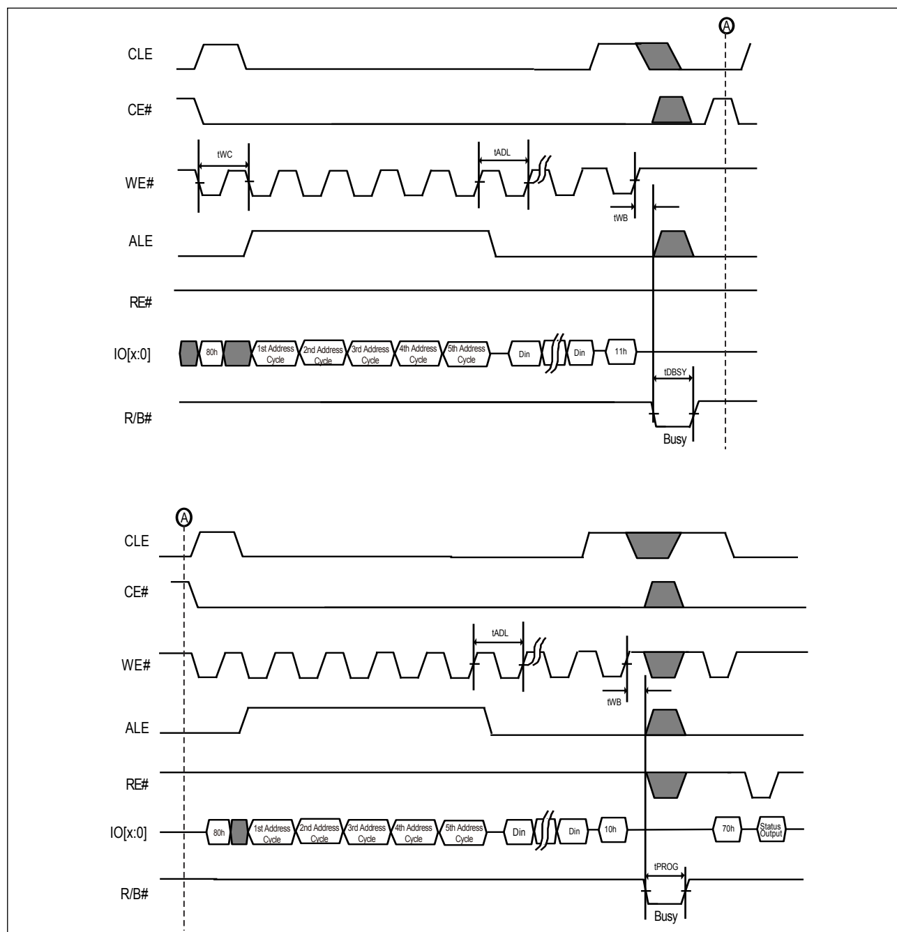
Figure 34-1. AC Waveforms for Two-plane Program (ONFI)
