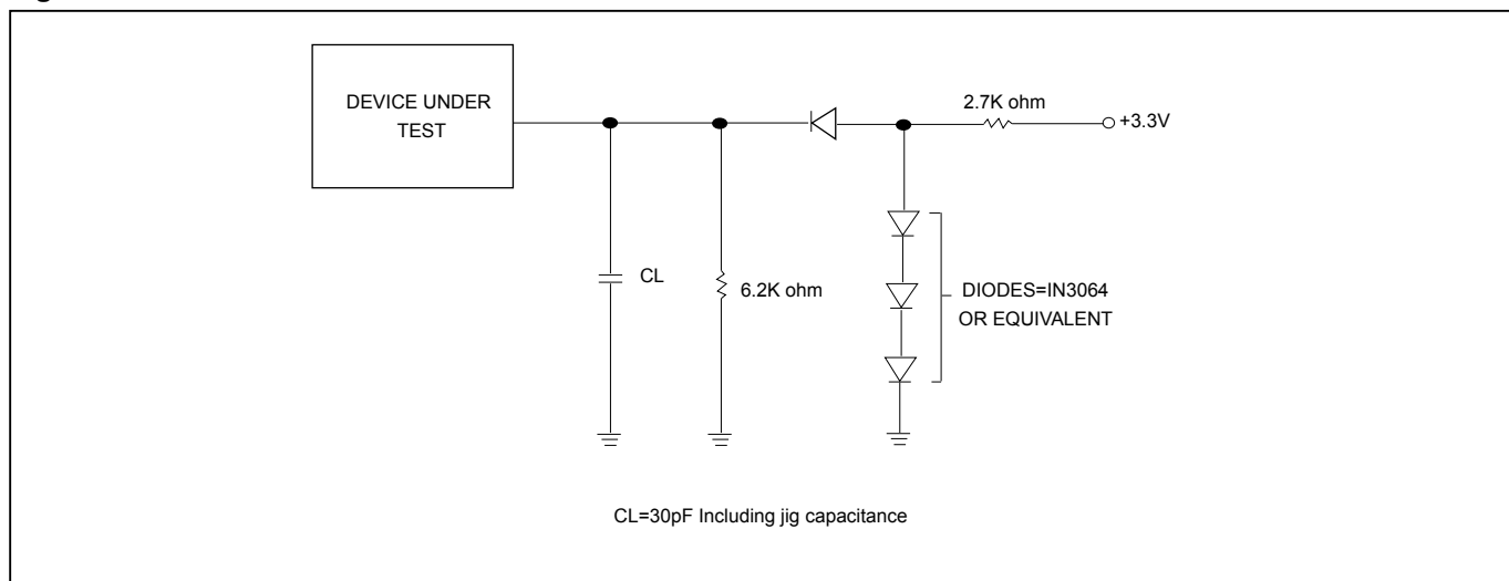
Figure 6. OUTPUT LOADING
