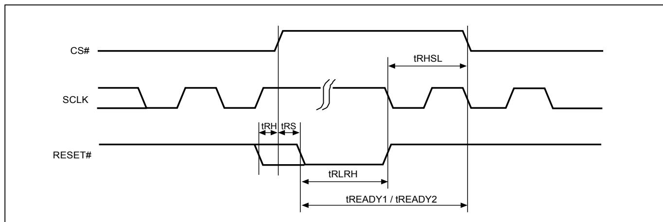
Figure 71. RESET Timing
