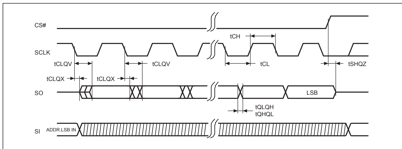
Figure 7. Output Timing
