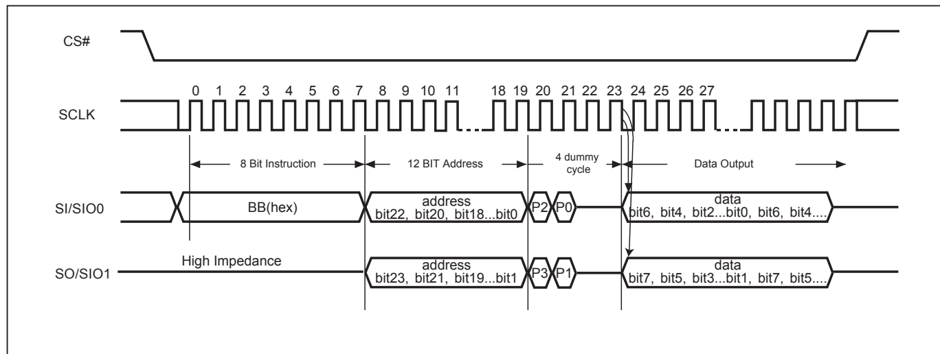
Figure 16. 2 x I/O Read Mode Sequence (Command BB)
