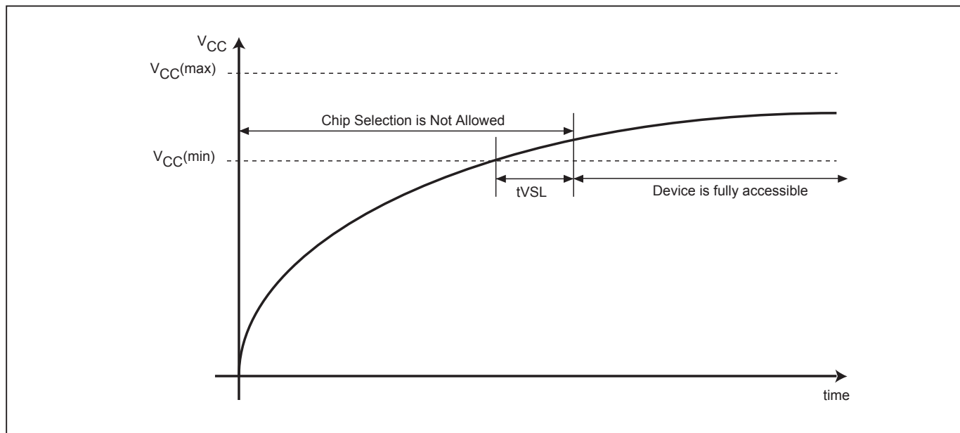
Figure 39. Power-up Timing
