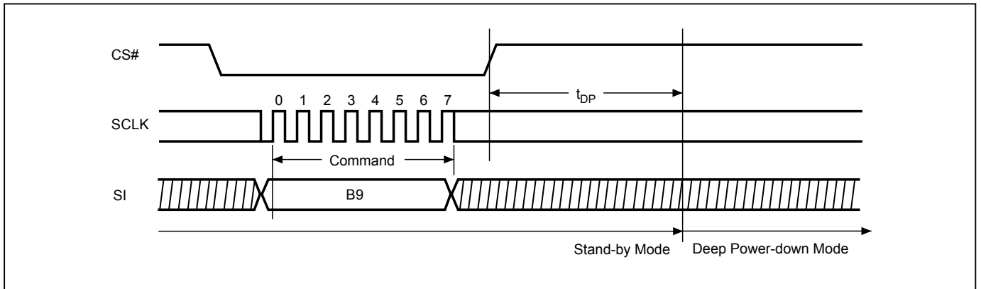
Figure 29. Deep Power-down (DP) Sequence (Command B9)
