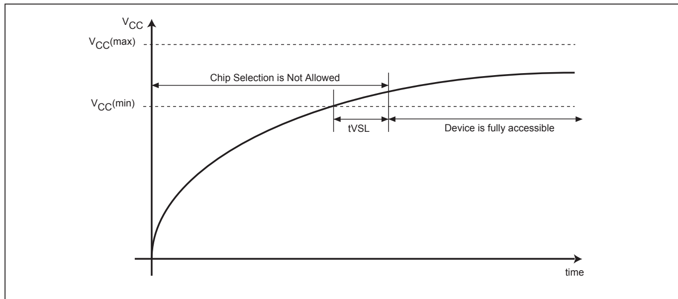
Figure 31. Power-up Timing
