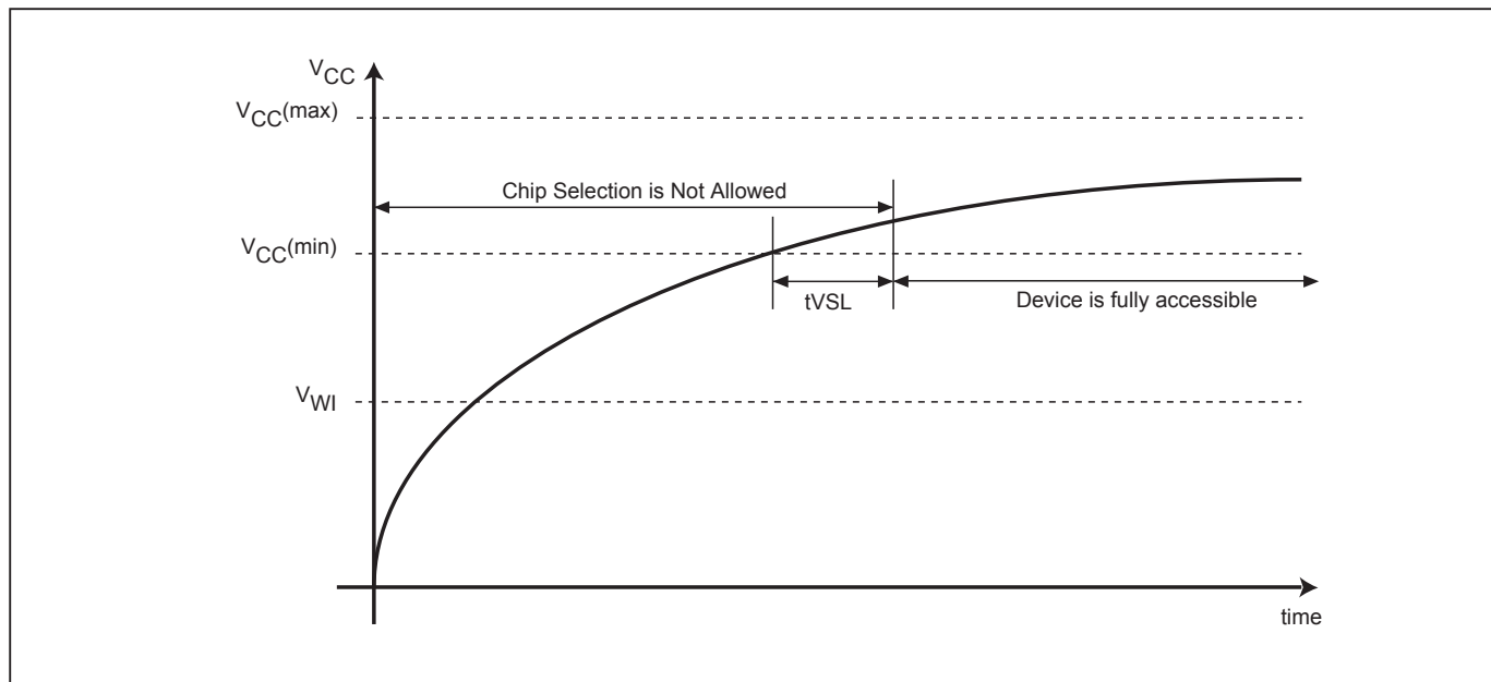
Figure 85. Power-up Timing
