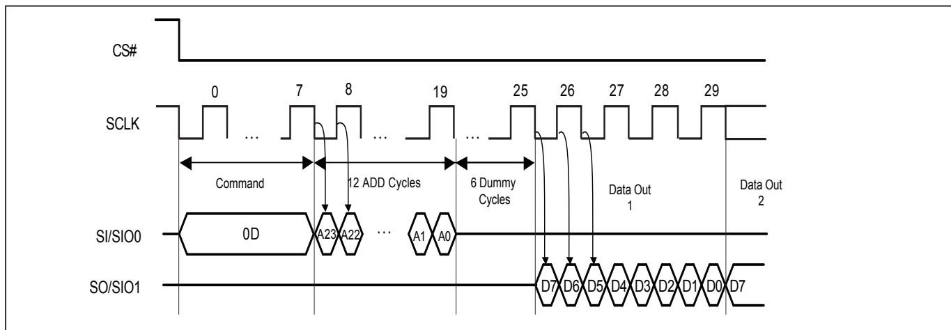
Figure 17. Fast DT Read (FASTDTRD) Sequence (Command 0D)
