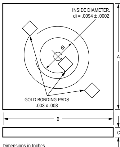
DIMENSIONS: INCHES
