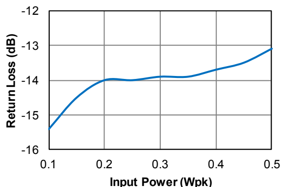
Return Loss vs. Input Power
