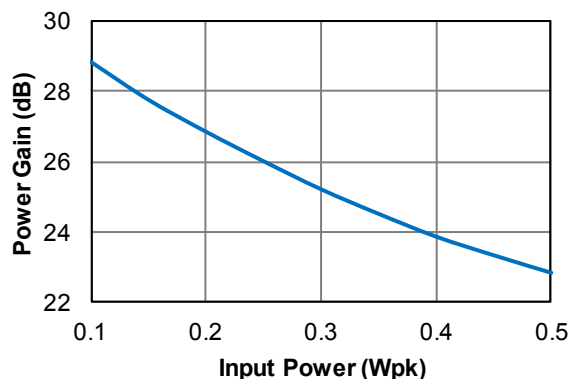
Power Gain vs. Input Power
