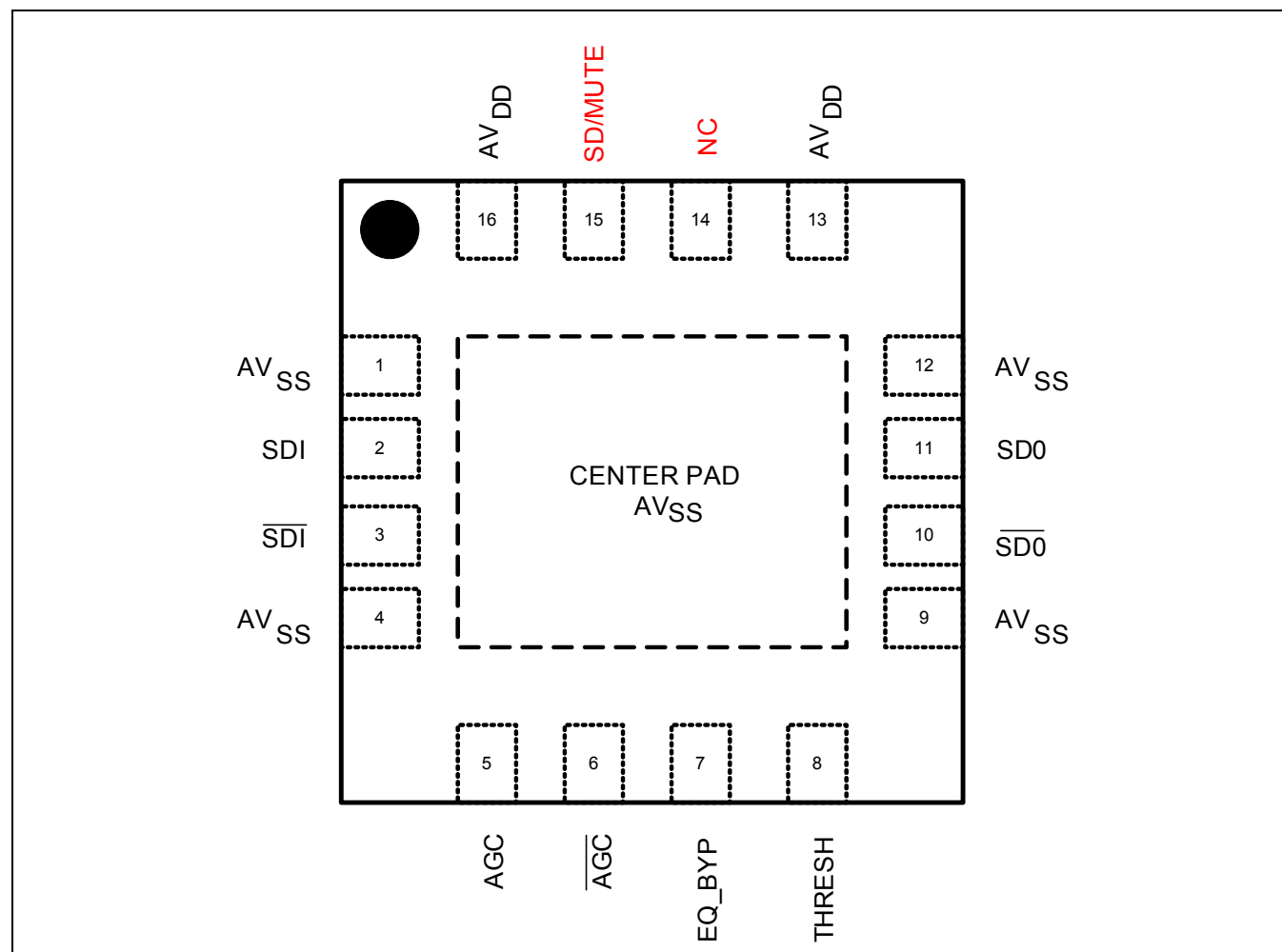
Figure 1-2. M21324 Pin Assignments
