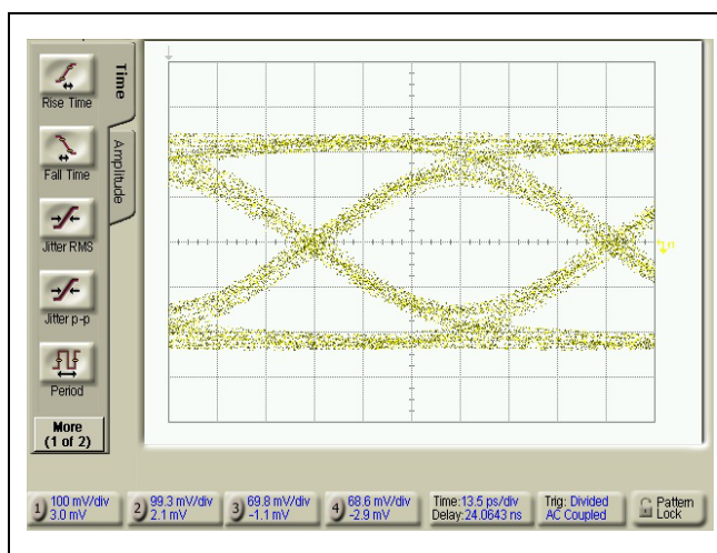
Figure 2-4. Eye Diagram at 12 Gbps, 2 dB of De-emphasis
