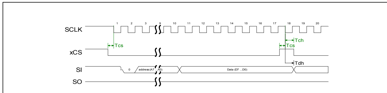
Figure 1-3. Serial Interface Random Write
