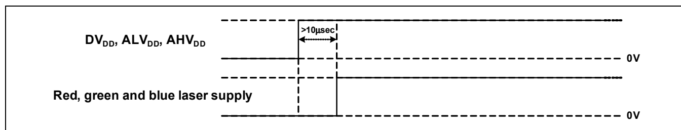
Figure 2-3. Power-Up
