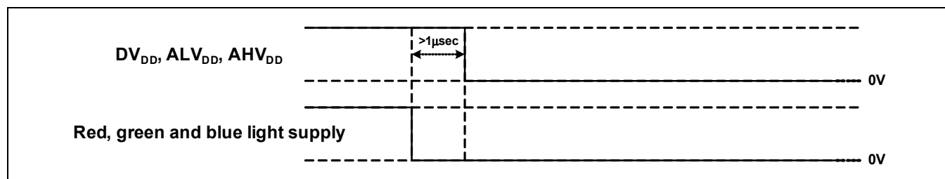
Figure 2-4. Power-Down
