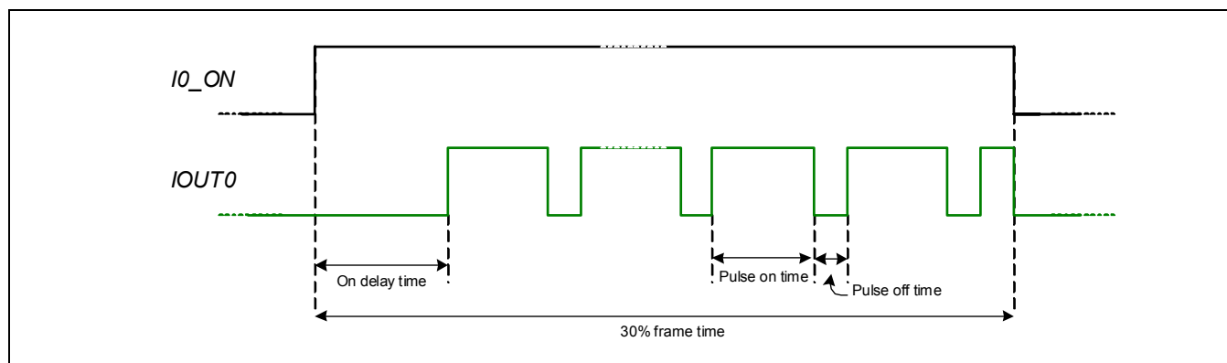
Figure 2-2. Multi Pulse Generator Timing
