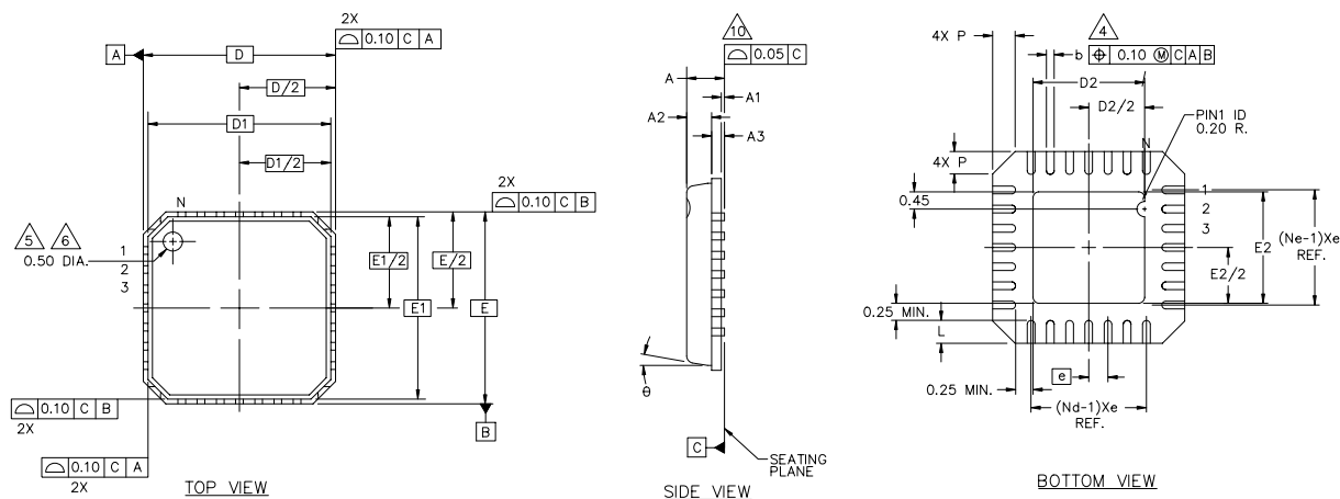
Figure 5-1. QFN32 Package Information
