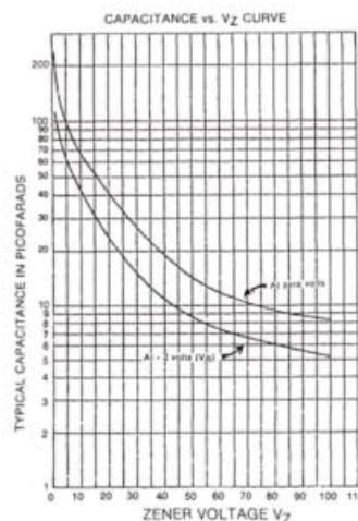
FIGURE 3 CAPACITANCE vs. ZENER VOLTAGE (TYPICAL)
