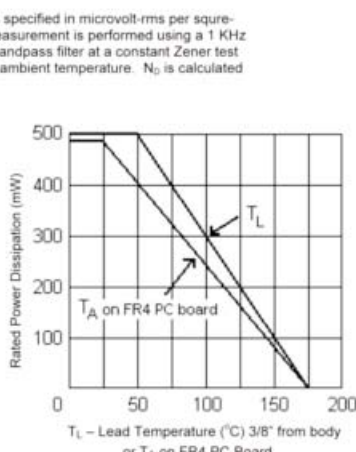
FIGURE 2 - POWER DERATING CURVE
