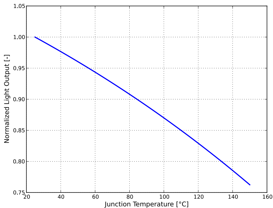
Figure 2. Typical normalized light output vs. junction temperature for LUXEON HR30 at 150mA.
