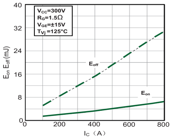
Figure 5: Switching Energy vs. Collector Current
