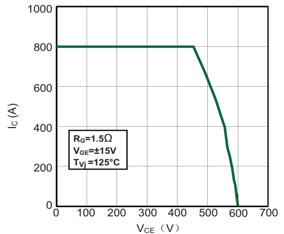
Figure 6: Reverse Biased Safe Operating Area
