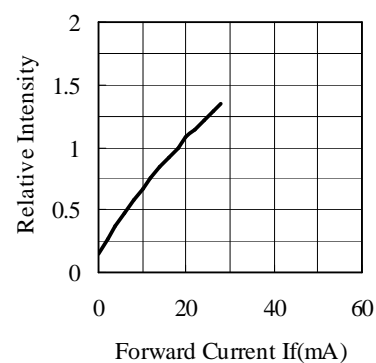
Forward Current vs. Relative Luminous Intensity
