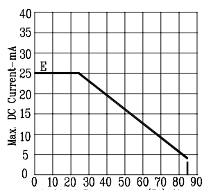
Fig8. MAX. ALLOWABLE DC CURRENT VS. AMBIENT TEMPERATURE.
